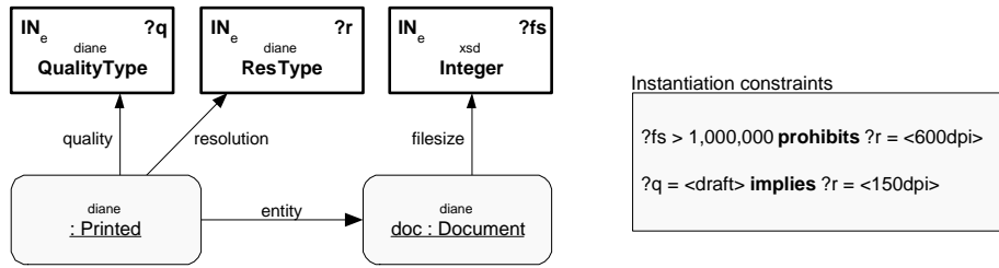
Fig. 10. Restricting several non-orthogonal variables by introducing variable names and an external dependencies list.
